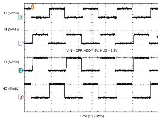
Figure 4. HS tied to GND Showing LI, HI, LO, and HO Signals
