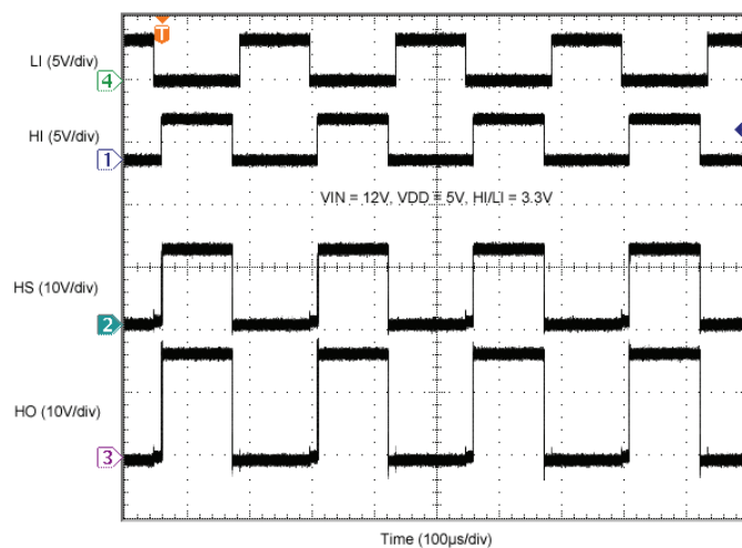
Figure 2. 4kHz Motor Operation Showing LI, HI, HS, and HO Signals
